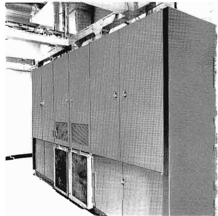
Rear of amplifier and control cabinets. Filters at bottom center are intakes for the two blowers which cool the entire transmitter. The room is air conditioned, with positive pressure to pull cool air through the transmitters.
