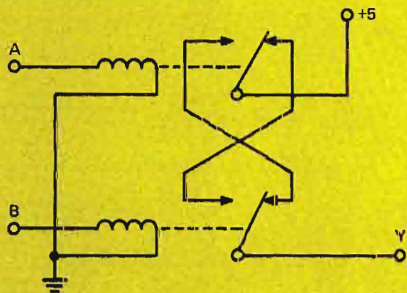
Figure 14. Two-Relay Version of Exclusive OR Circuit.
