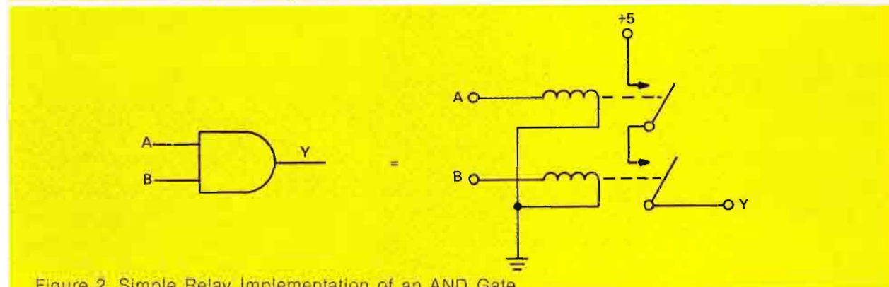
Figure 2. Simple Relay Implementation of an AND Gate.
