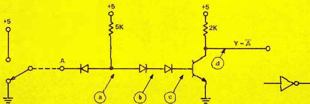
Figure 17. Prototype DTL Inverter.
