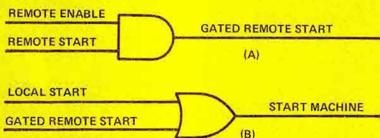
Figure 7. Typical Broadcast Machine-Control Applications of Logic Elements.
