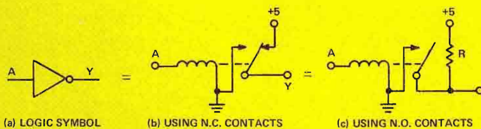
Figure 4. Simple Relay Implementations for an Inverter.
