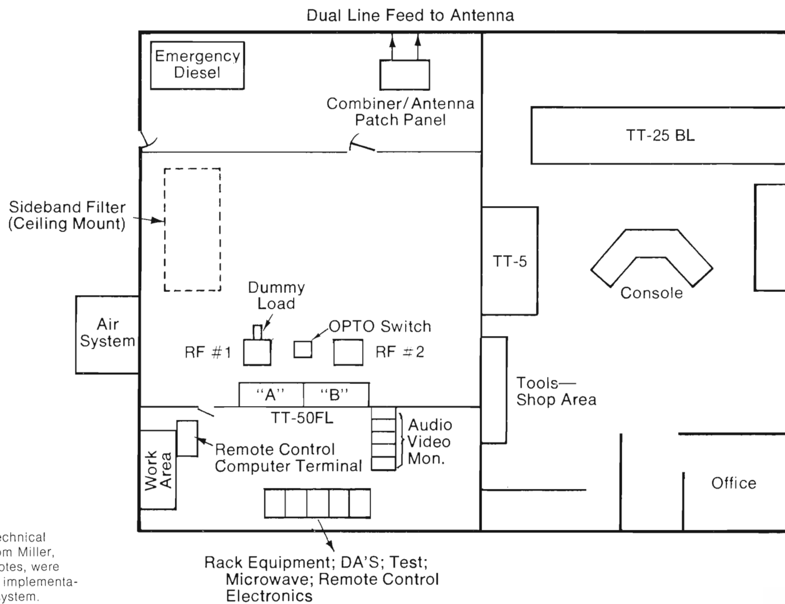
Layout, WKYC-TV Transmitting facility.
