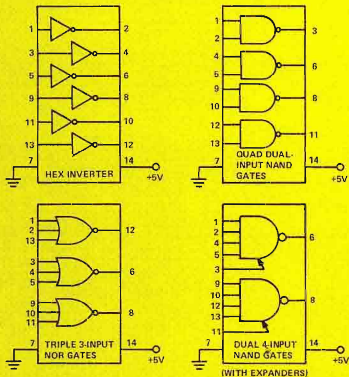
Figure 20. Typical Combinations of Gates in IC Packages.
