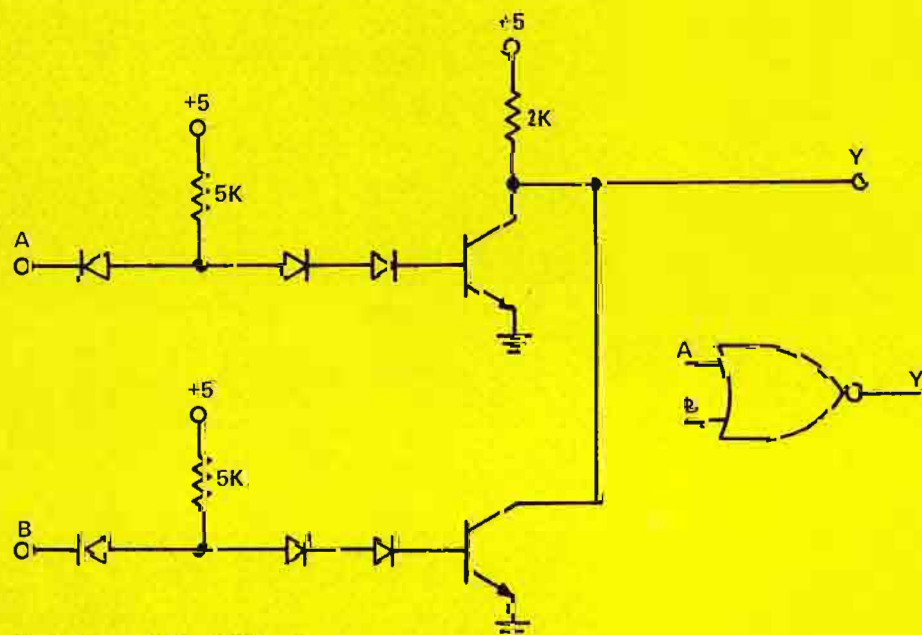
Figure 19. Prototype DTL NOR Gate.
