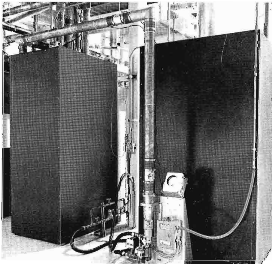
Rear of Opto-Switcher cabinet and one power supply cabinet. 50 kW water-cooled dummy load is positioned behind the power supply cabinet.
