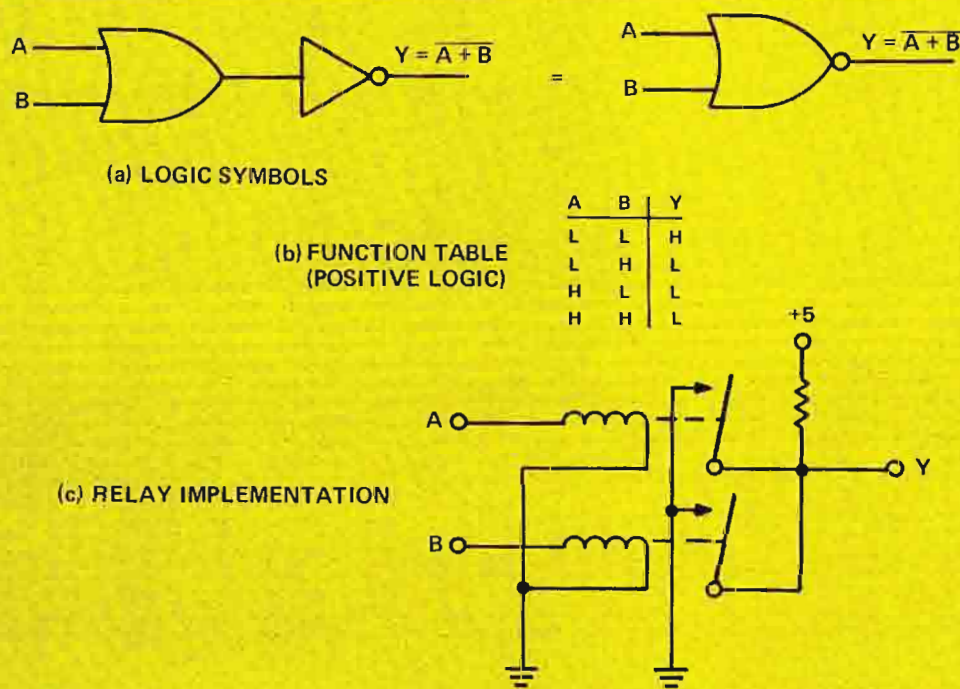
Figure 11. Two-Input NOR (NOT OR) Gates.
