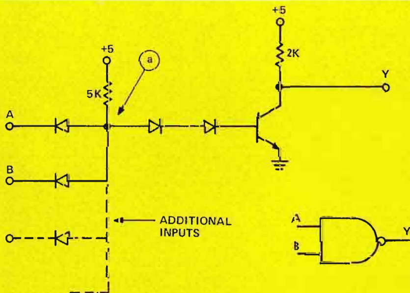
Figure 18. Prototype DTL NAND Gate.
