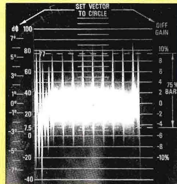
Differential Phase
