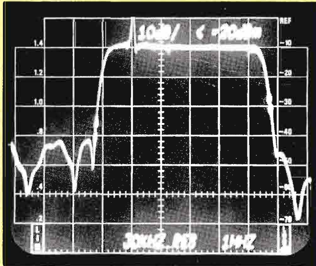
10 dB/vertical division
