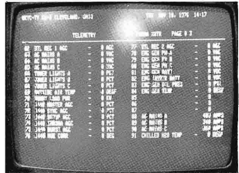
Computer-controlled system provides instant access to programmed transmitting system data. Telemetry, metering and numerous other system operating functions are available for display as "pages" on the video monitor.
