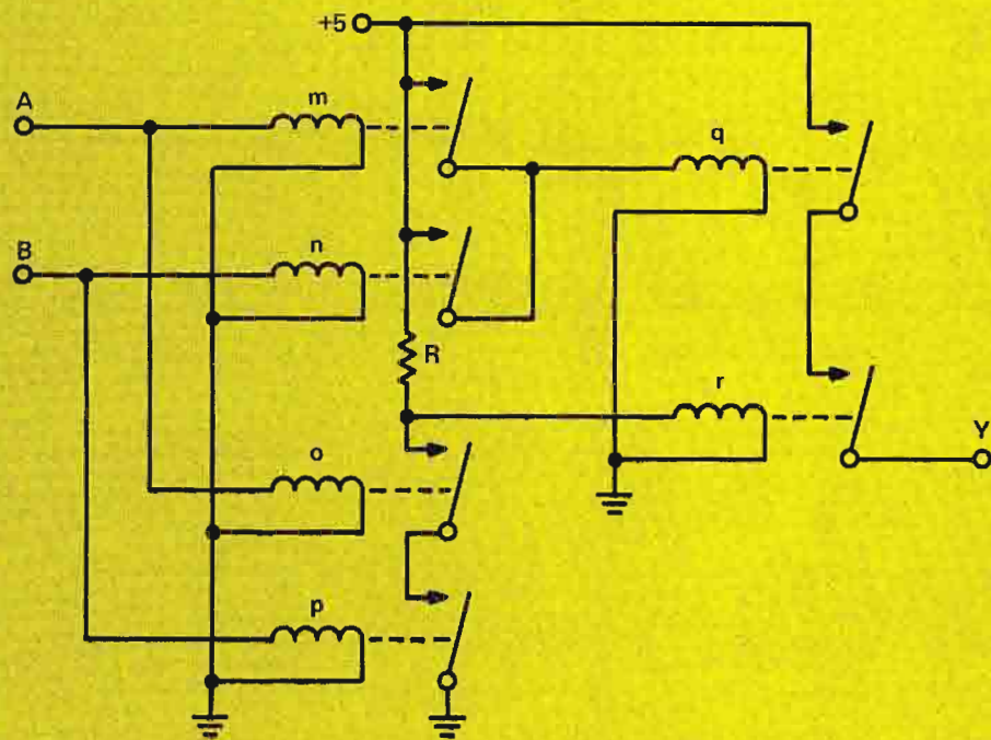
Figure 13. Possible Relay Implementation of Exclusive OR Function.
