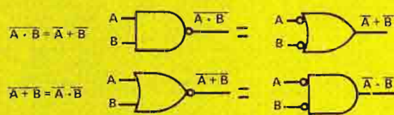
Figure 21. DeMorgan's Theorems.
