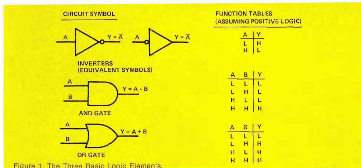
Figure 1. The Three Basic Logic Elements.
