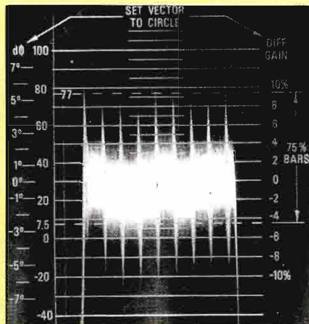
Differential Gain
