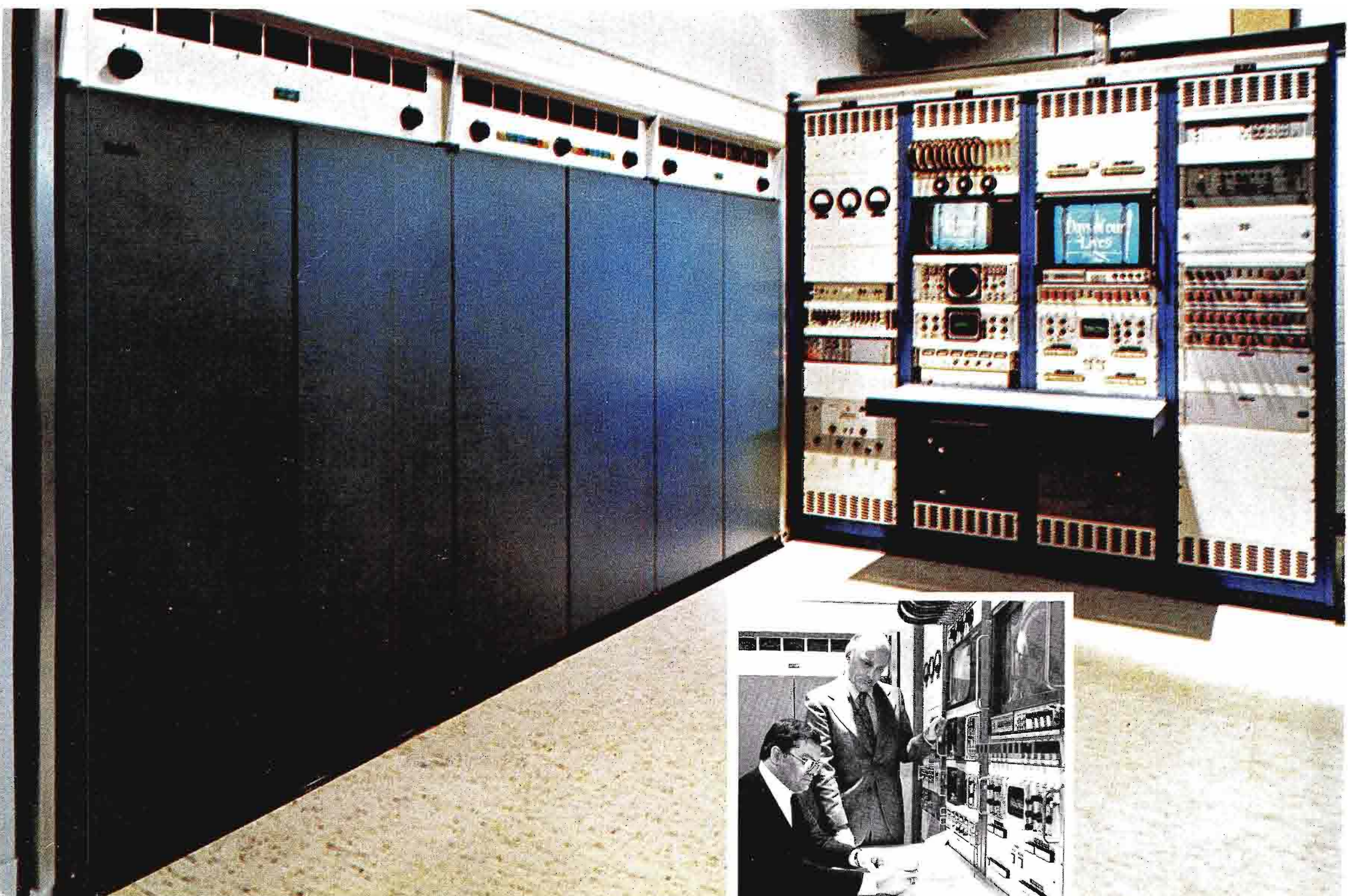
Front line cabinets of TT-50FL, 50 kW transmitter at WKYC-TV are built-in to form a wall of the control area. Extending at right angles to the transmitter are the audio and video monitoring racks.
