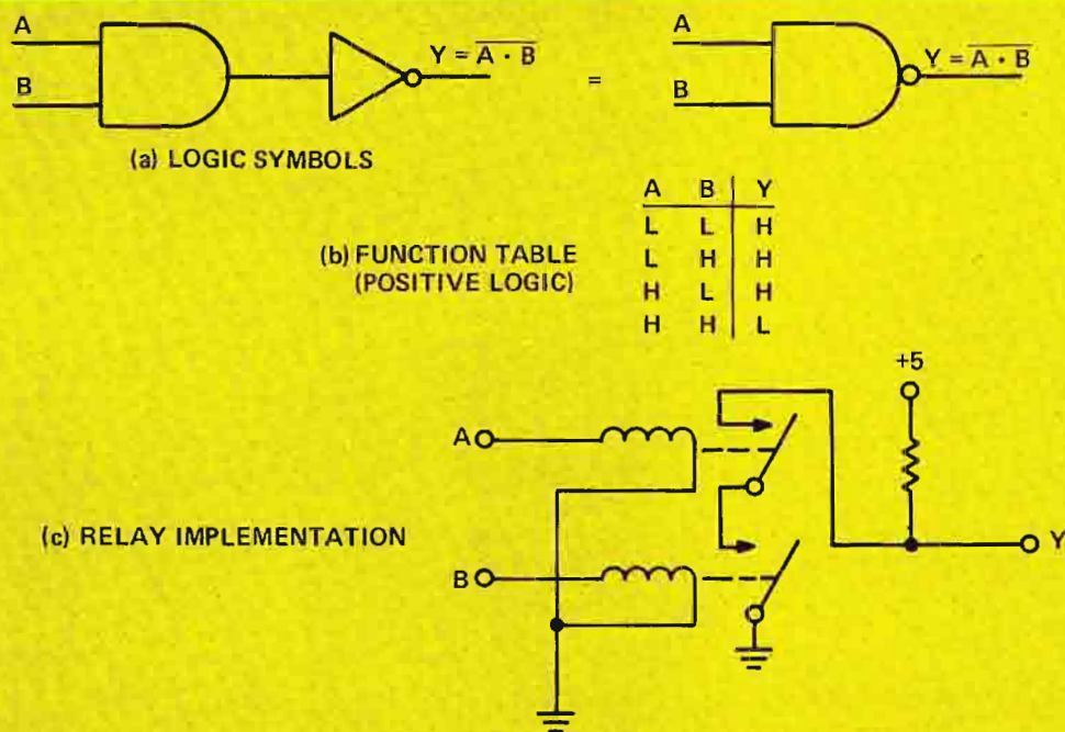
Figure 10. Two-Input NAND (NOT AND) Gate.
