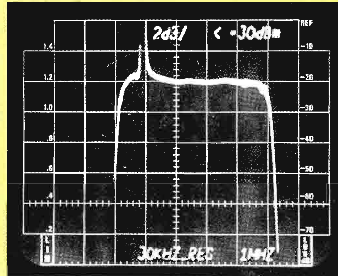
2 dB/vertical division
