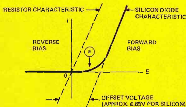
Figure 16. Silicon Diode Characteristic.
